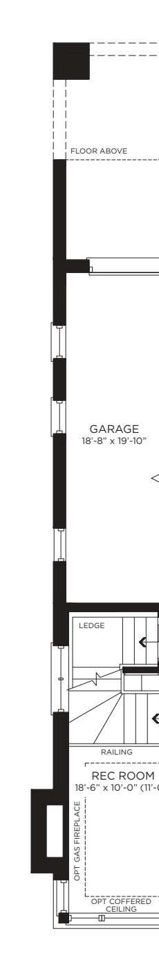
Partial Ground Floor Corner Unit
