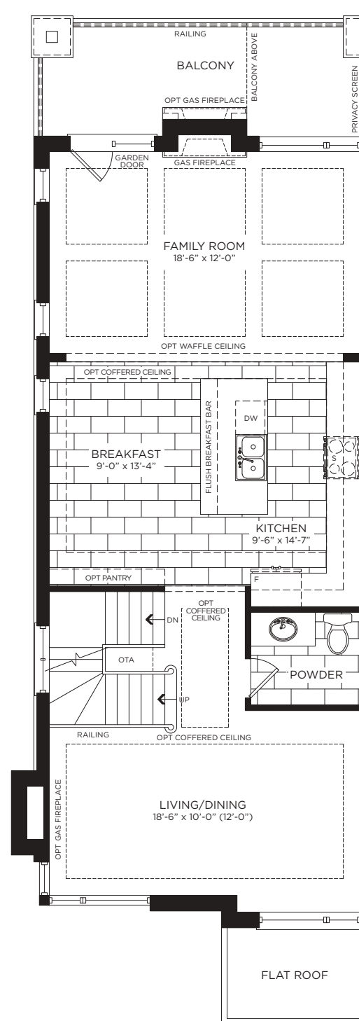
Main Floor End Unit
